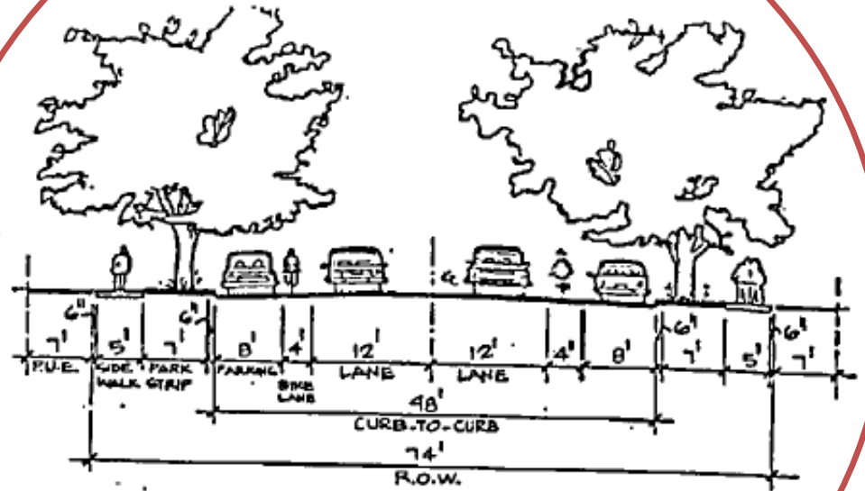
Collector 74' R-O-W
