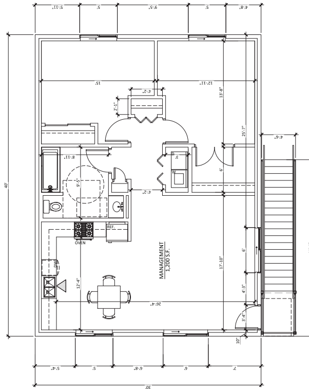
BUILDING "A" RESIDENCE 2ND FLOOR PLAN
