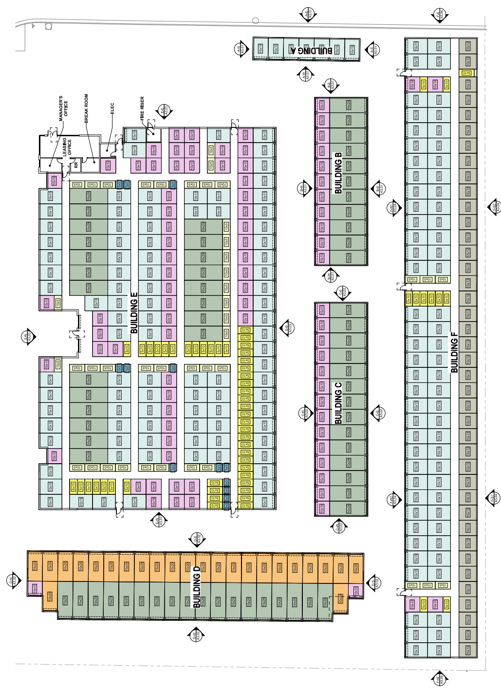
1 OVERALL UNIT PLAN - LEVEL 01
