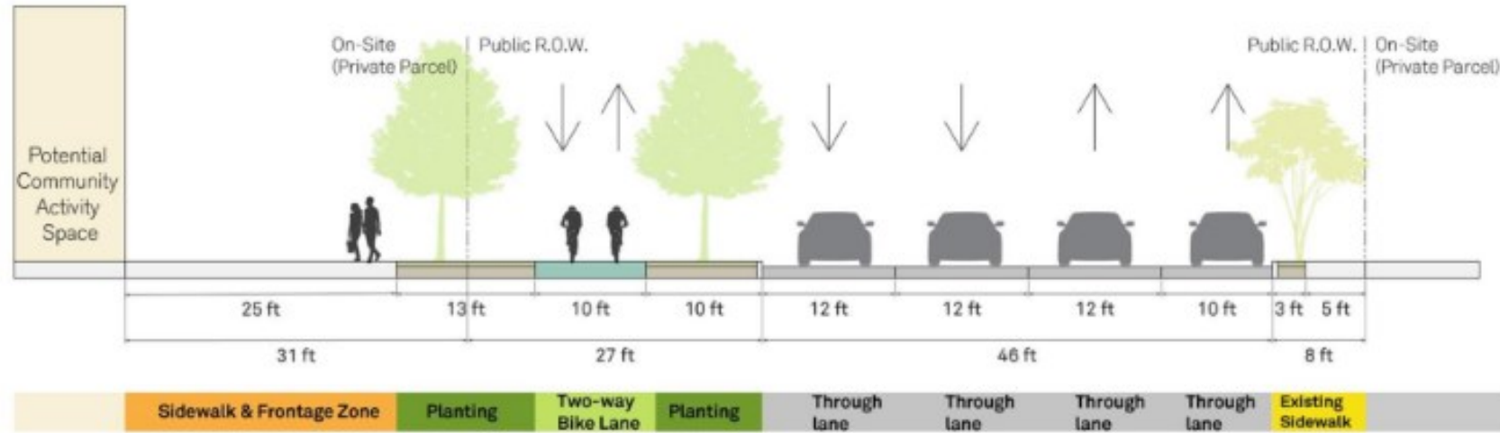
Cross Section- 16th Street
