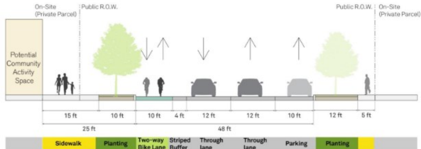
Cross Section- O Street
