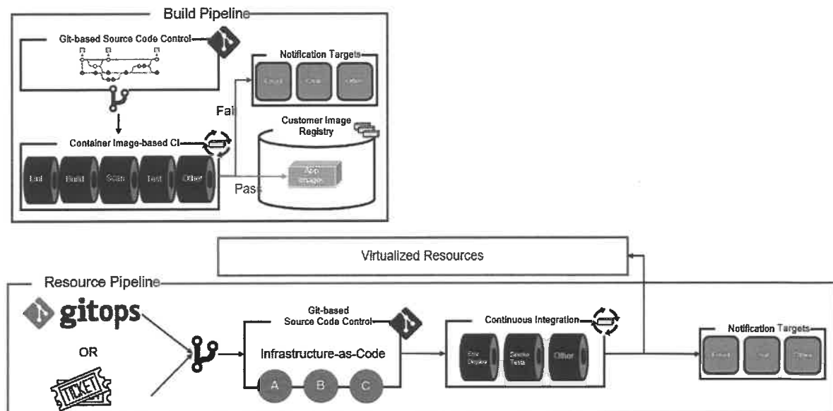
Figure 8: Virtual Platform & Cloud
