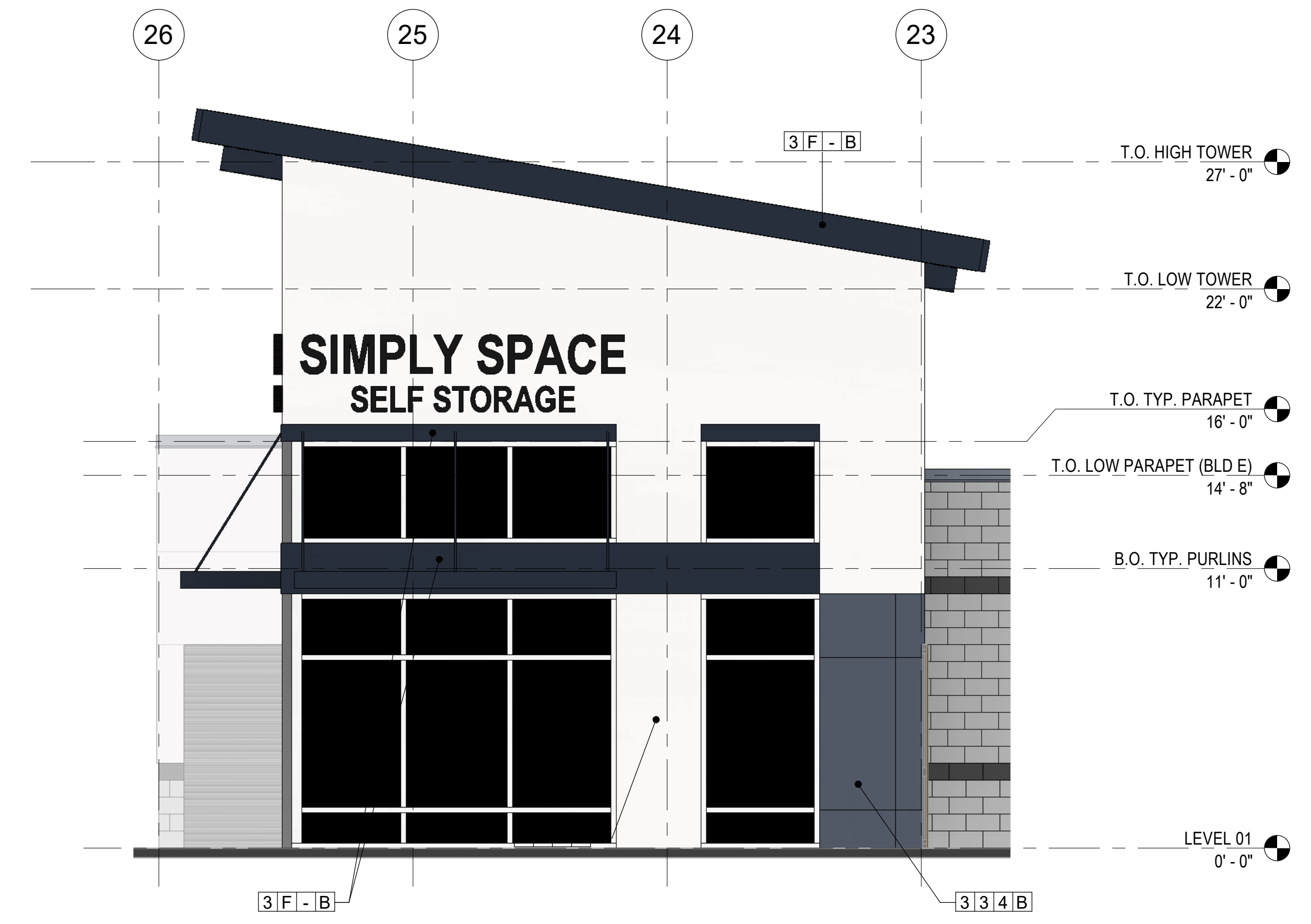
1 ENLARGED ELEVATION - BUILDING E ENTRY - NORTH 1/4" = 1'-0"
